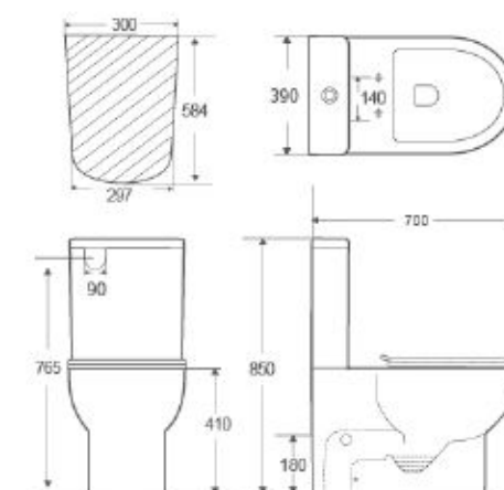
BL-116-TPT Washdown Flushing Toilet Size: 700×390×850mm P-trap: 180mm Roughing-in
