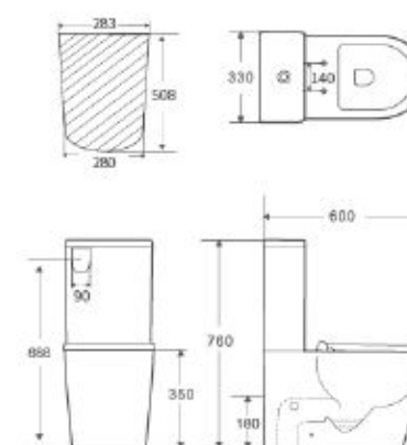
BL-JUNIOR Junior Toilet Suite (Tornado Rimless) Size: 600x330x760mm P-trap: 180mm Roughing-in
