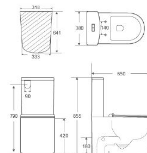
BL-THRONE Extra length Toilet Suite Size: 650×380×855mm P-trap: 180mm Roughing-in
