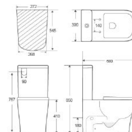
BL-107-TPT Pure Rimless Toilet Suite (New) Size: 680×390×850mm P-trap: 180mm Roughing-in
